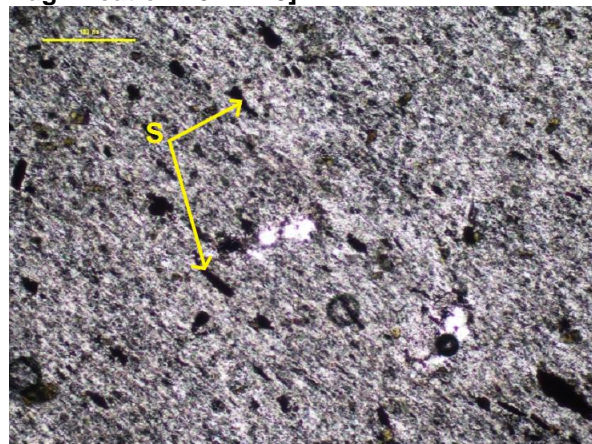
Fig. 16 Blebs Of Ore Minerals Oriented Along With Gangue Minerals In A Fine Grained Rock. [S- Sulphide Minerals, XPL, Magnification 10X × 10]
